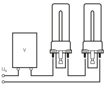
Circuit diagram
