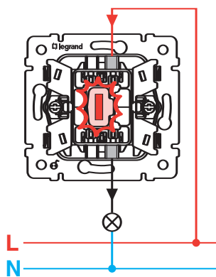
STD 1L
