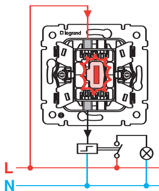
STD 1PL
