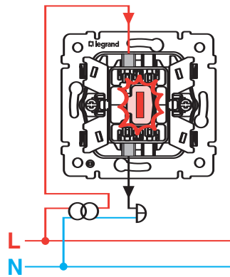
STD 1PLE
