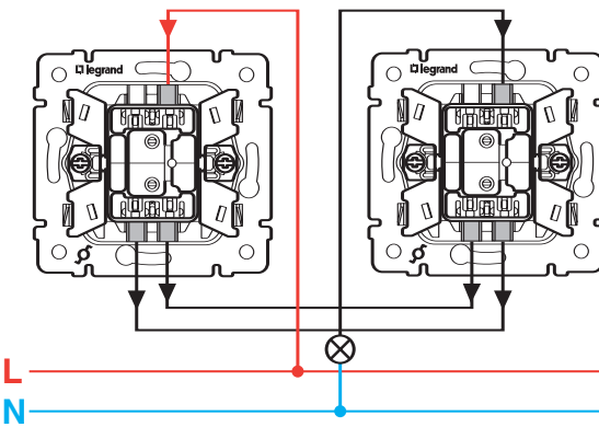
STD 6 - 6 IP44
